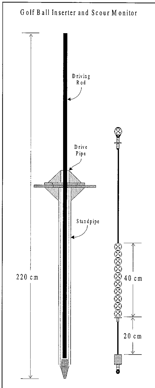
Figure 1. Diagram of a standard golf ball type scour monitor inserter and monitor.
